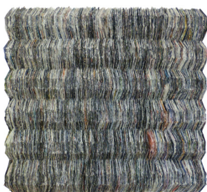
Relief: crap
